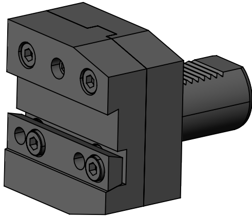
90 DEGREE VDI40 STATIC TOOL OUTPUT: 26mm BLADE COOLANT: EXTERNAL
